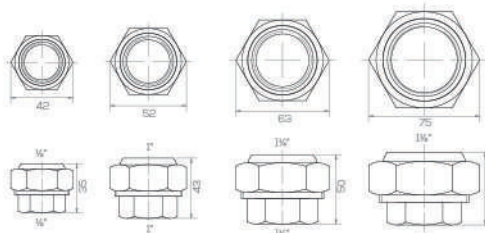
SW model *15° adjustability
