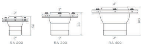
SW model *15° adjustability
