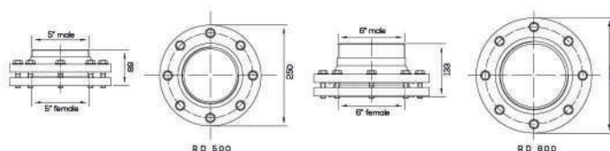
SW model Heavy Duty *5° adjustability for 6 & "5"
